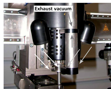
Fume exhaust
